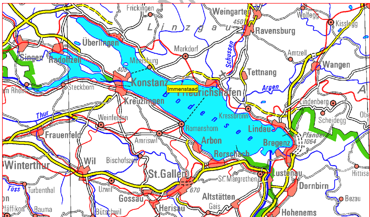
Figure 5: 3800 - 4200 MHz satellite earth station in neighbouring country requiring protection
