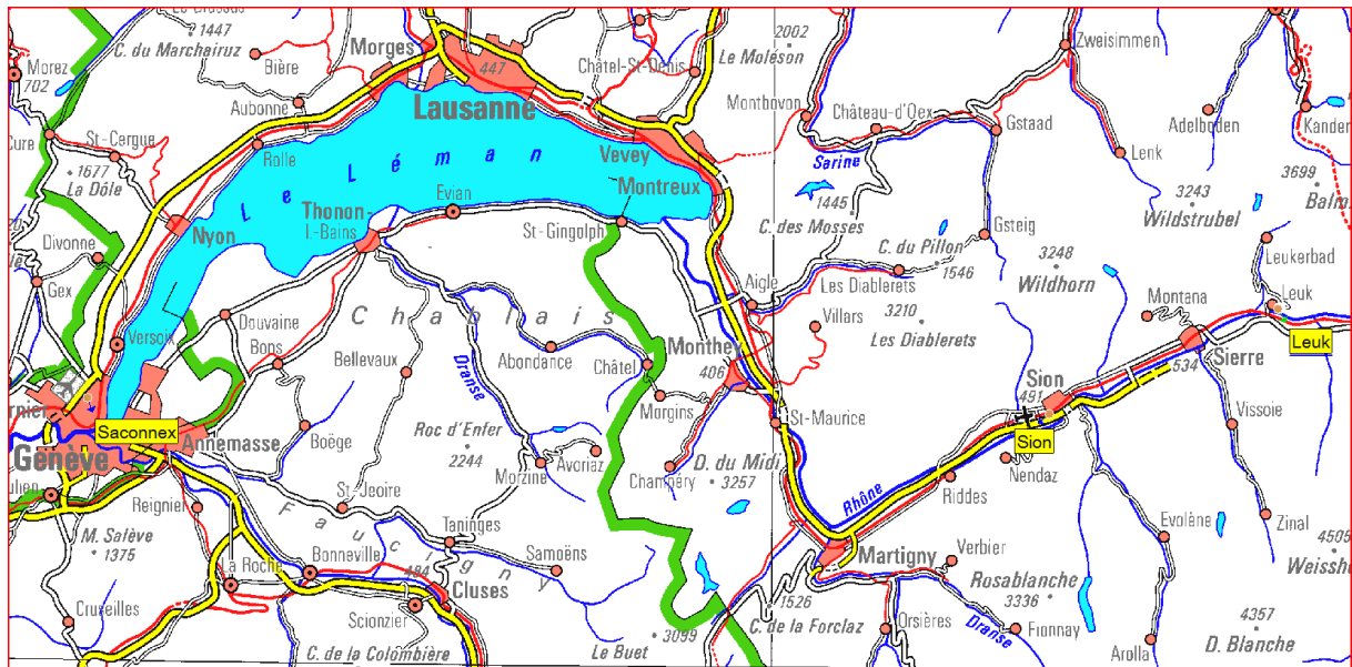
Figure 4: 3600 - 4200 MHz satellite earth stations in Switzerland requiring protection.
