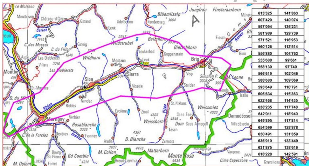
Figure 6: Protection zone in Valais for the 3640 - 3800 MHz frequency range
